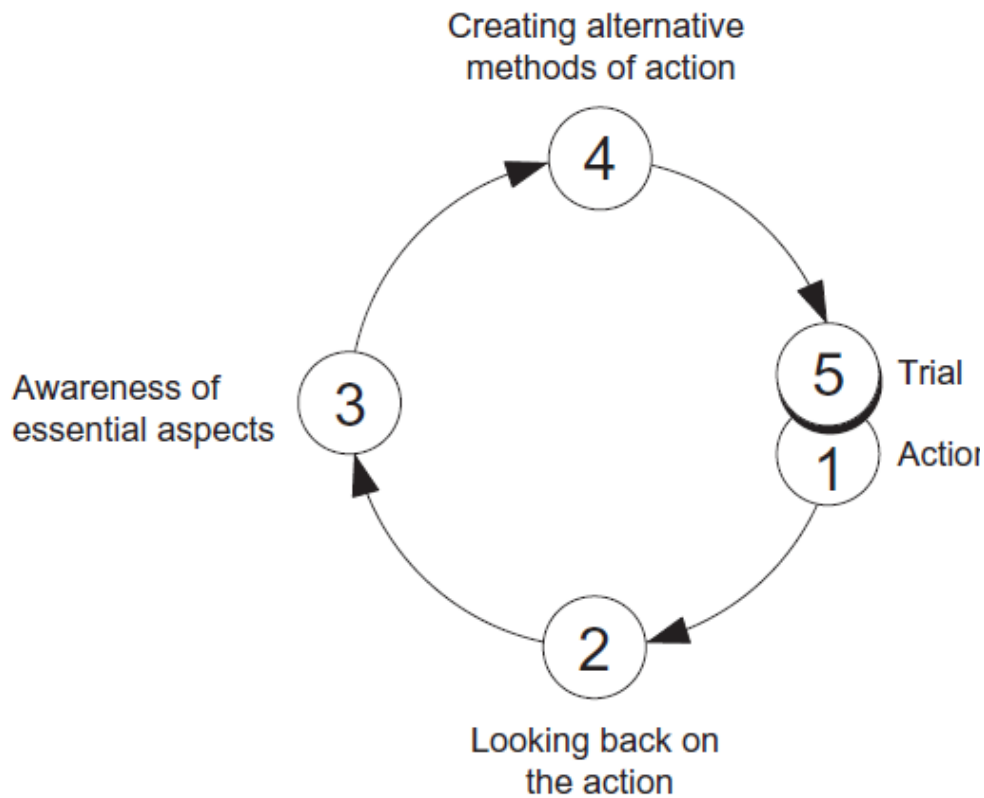
ALACT-model
